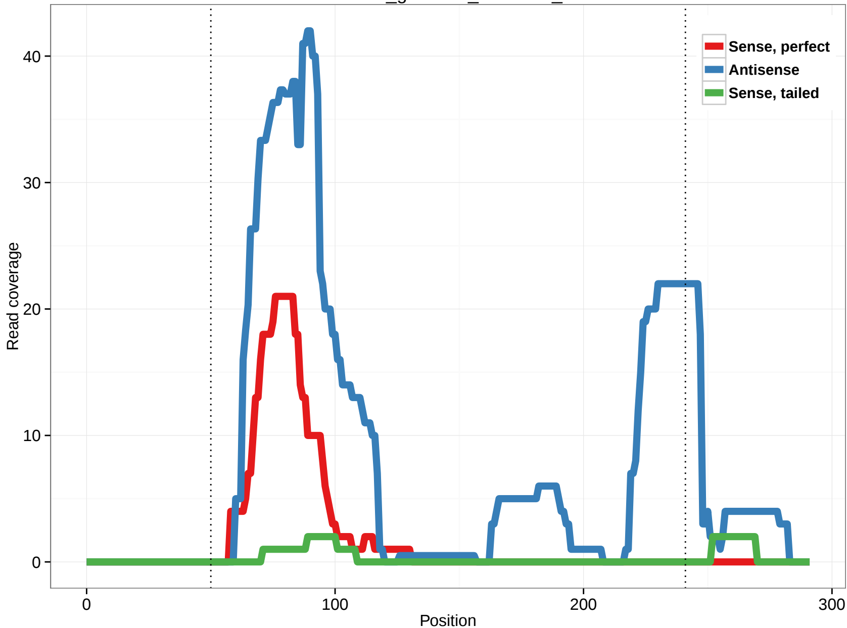
rheMac3_genscan_chr10.15_40
