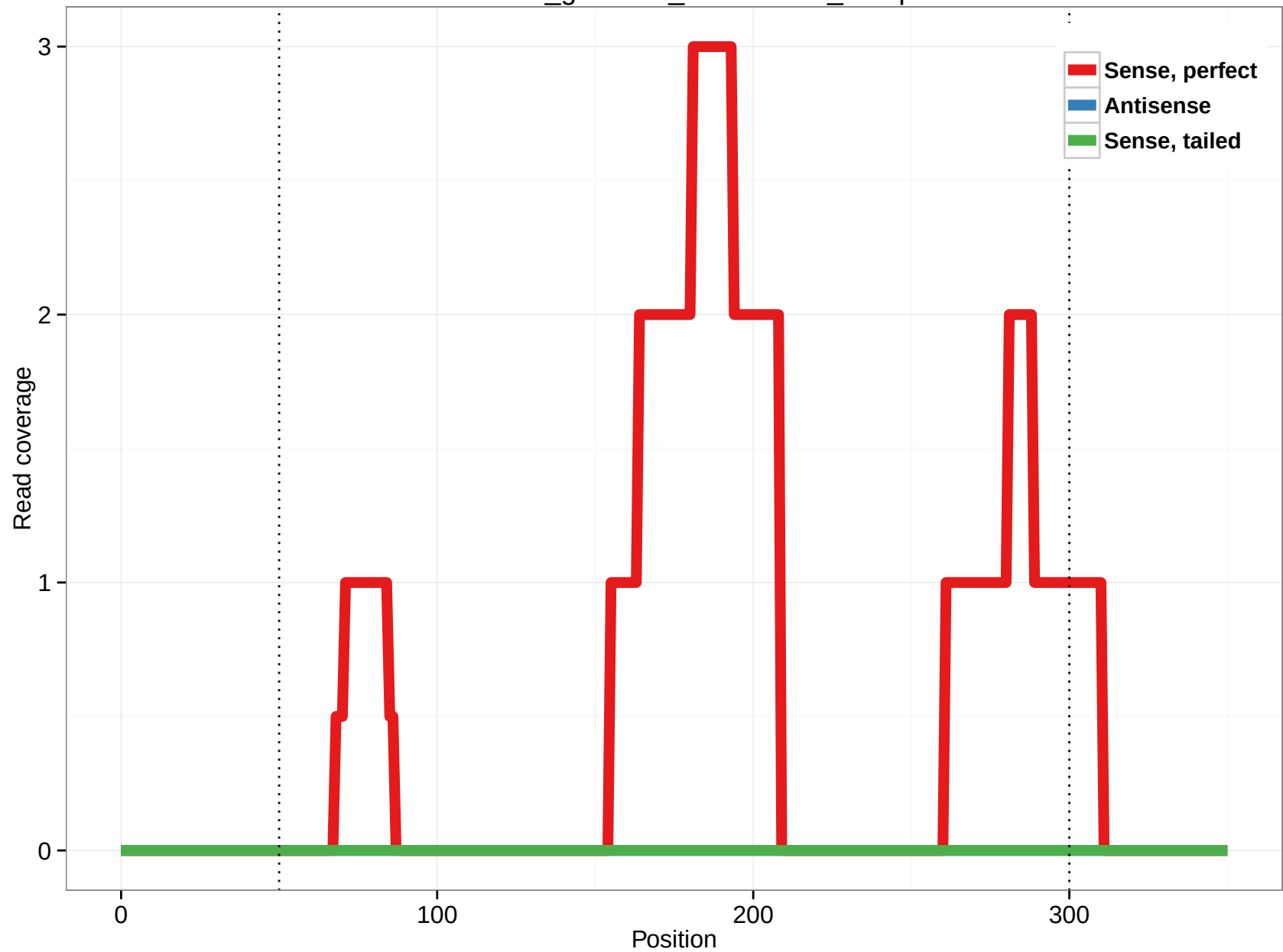
rheMac3_genscan_chr10.1599_13.5p
