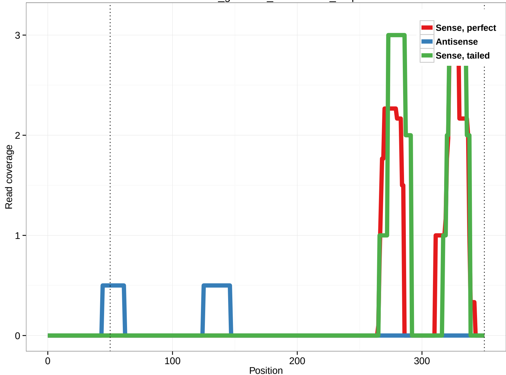
rheMac3_genscan_chr10.1580_6.5p
