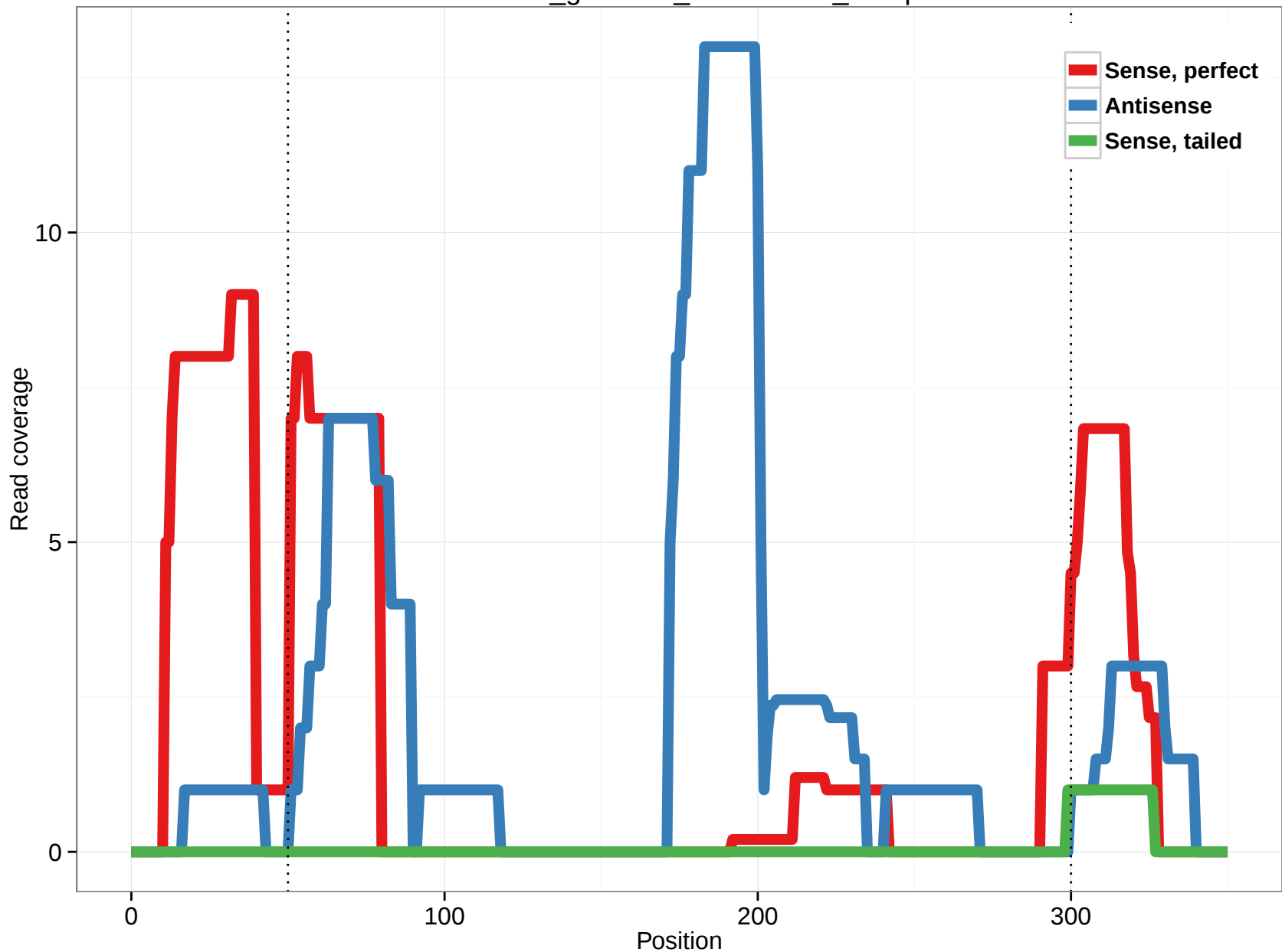
rheMac3_genscan_chr10.1580_50.5p
