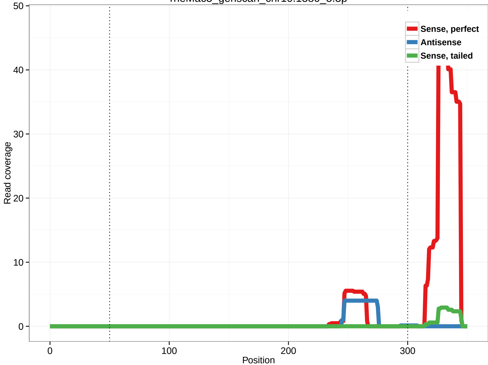
rheMac3_genscan_chr10.1580_5.3p
