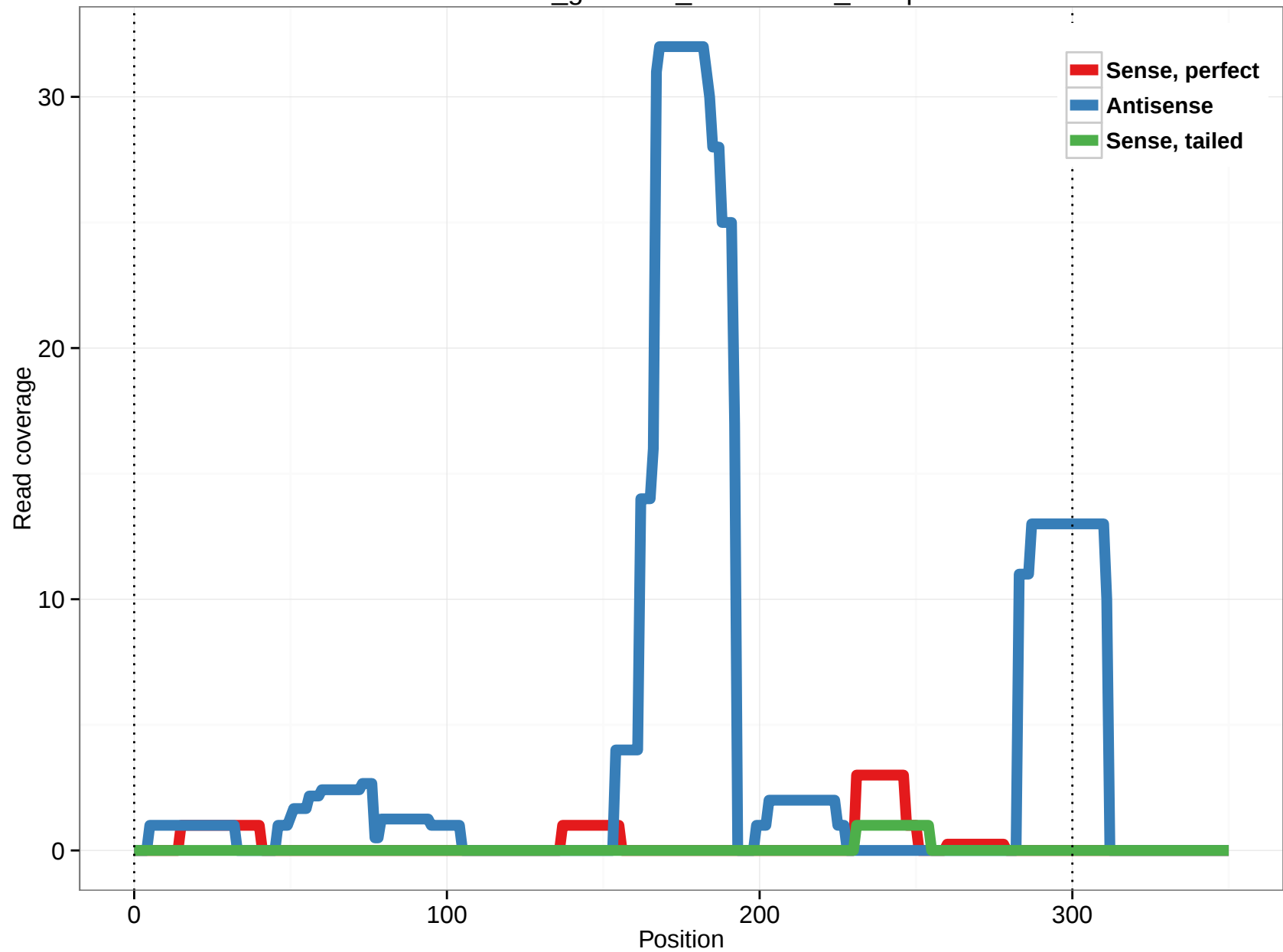
rheMac3_genscan_chr10.1580_49.3p
