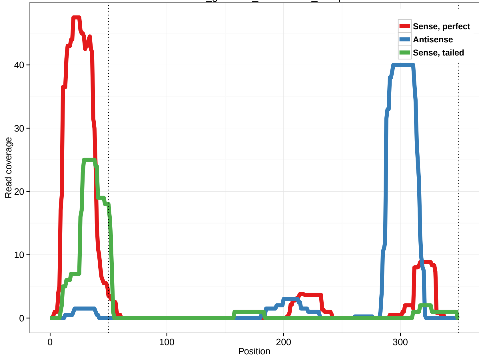
rheMac3_genscan_chr10.1580_47.5p
