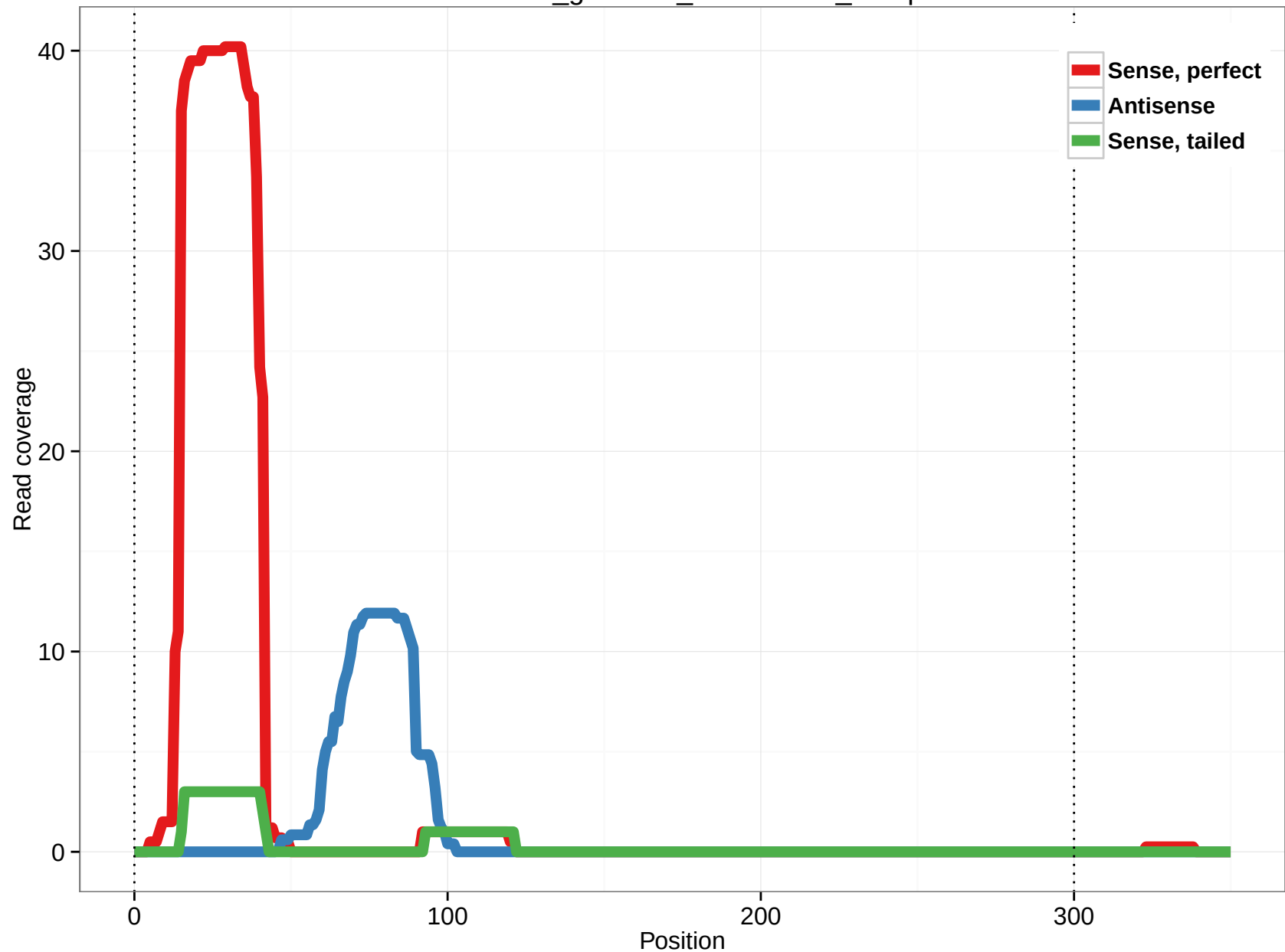
rheMac3_genscan_chr10.1580_43.3p
