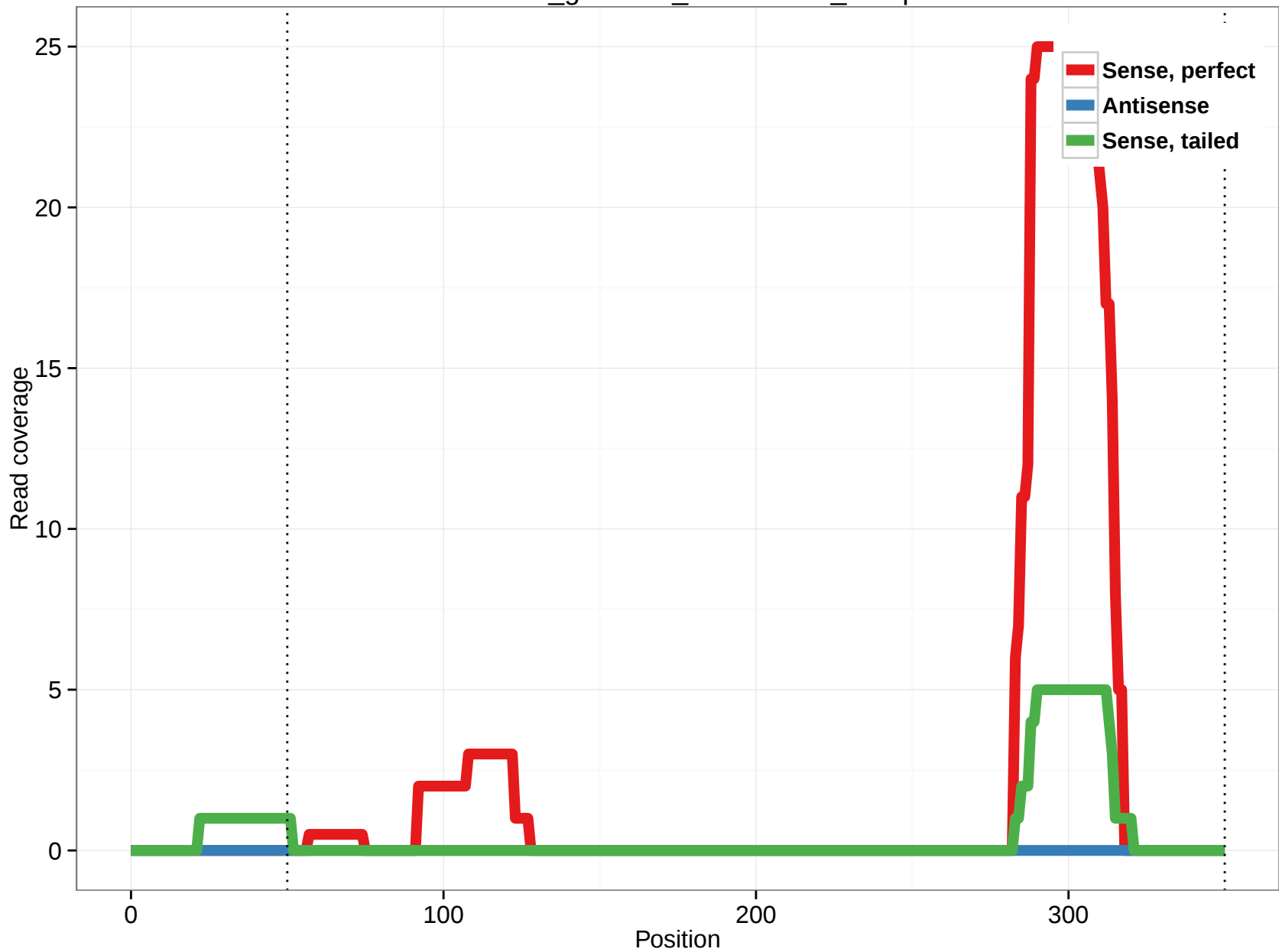
rheMac3_genscan_chr10.1580_32.5p
