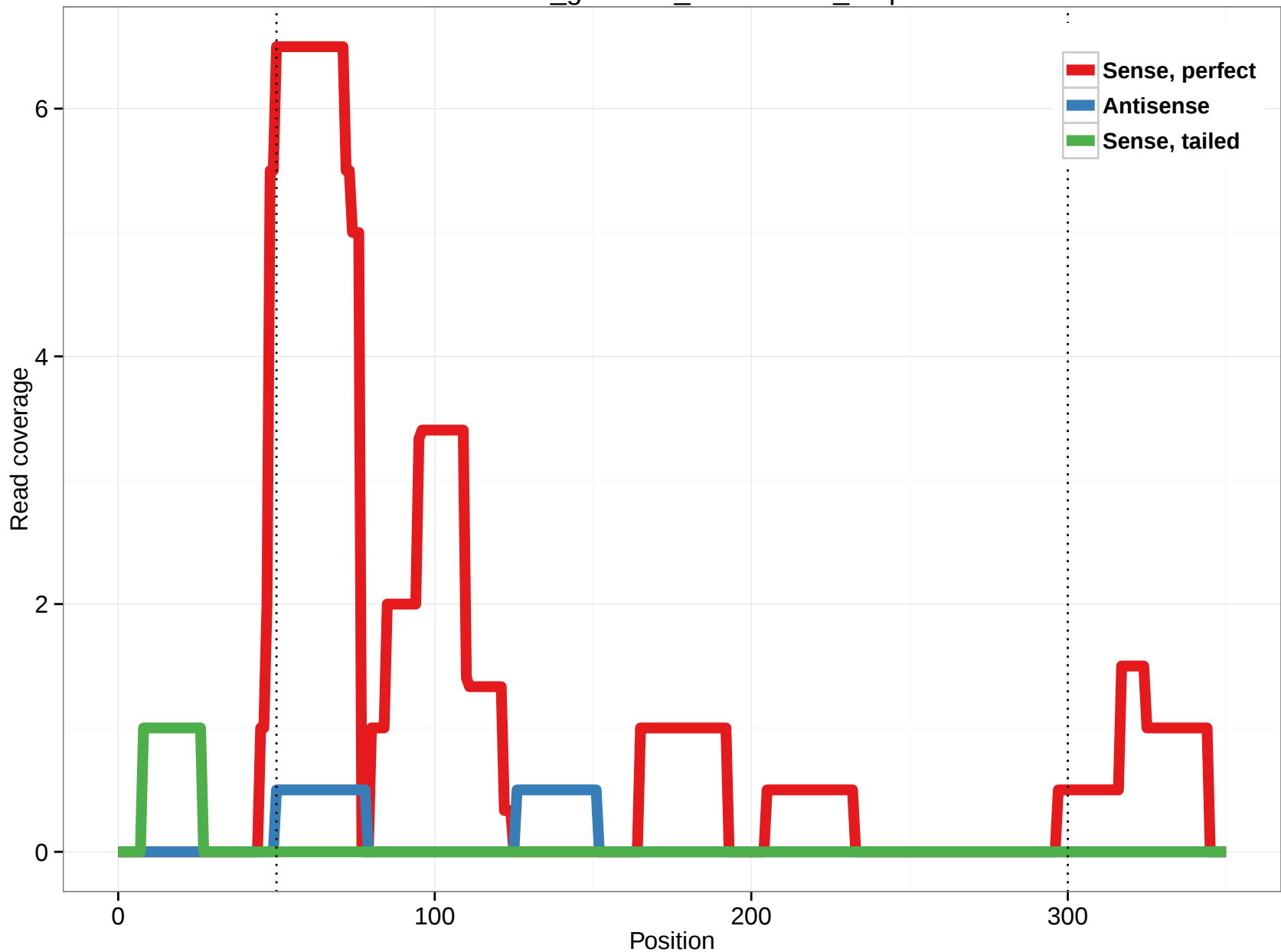
rheMac3_genscan_chr10.1570_8.5p
