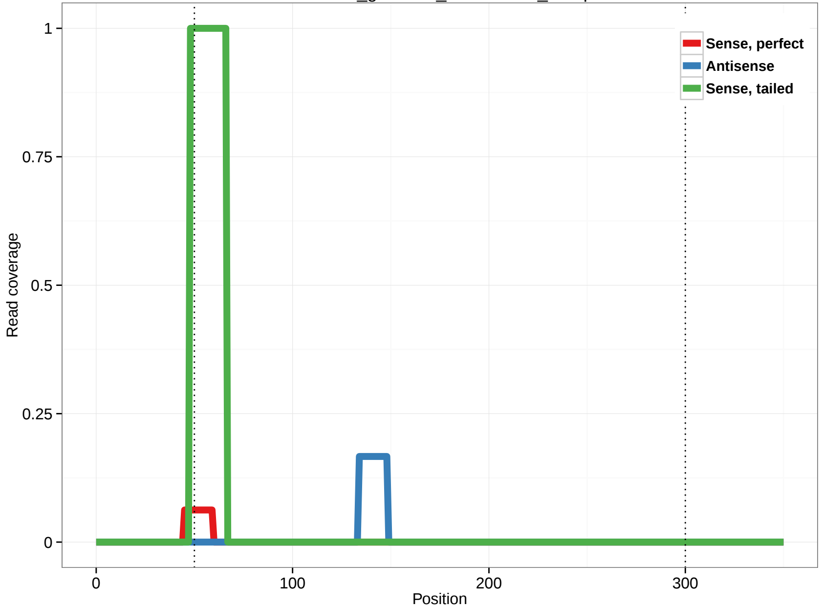
rheMac3_genscan_chr10.1566_22.3p
