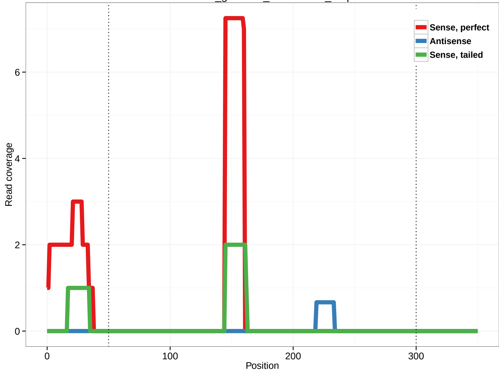
rheMac3_genscan_chr10.1564_3.5p
