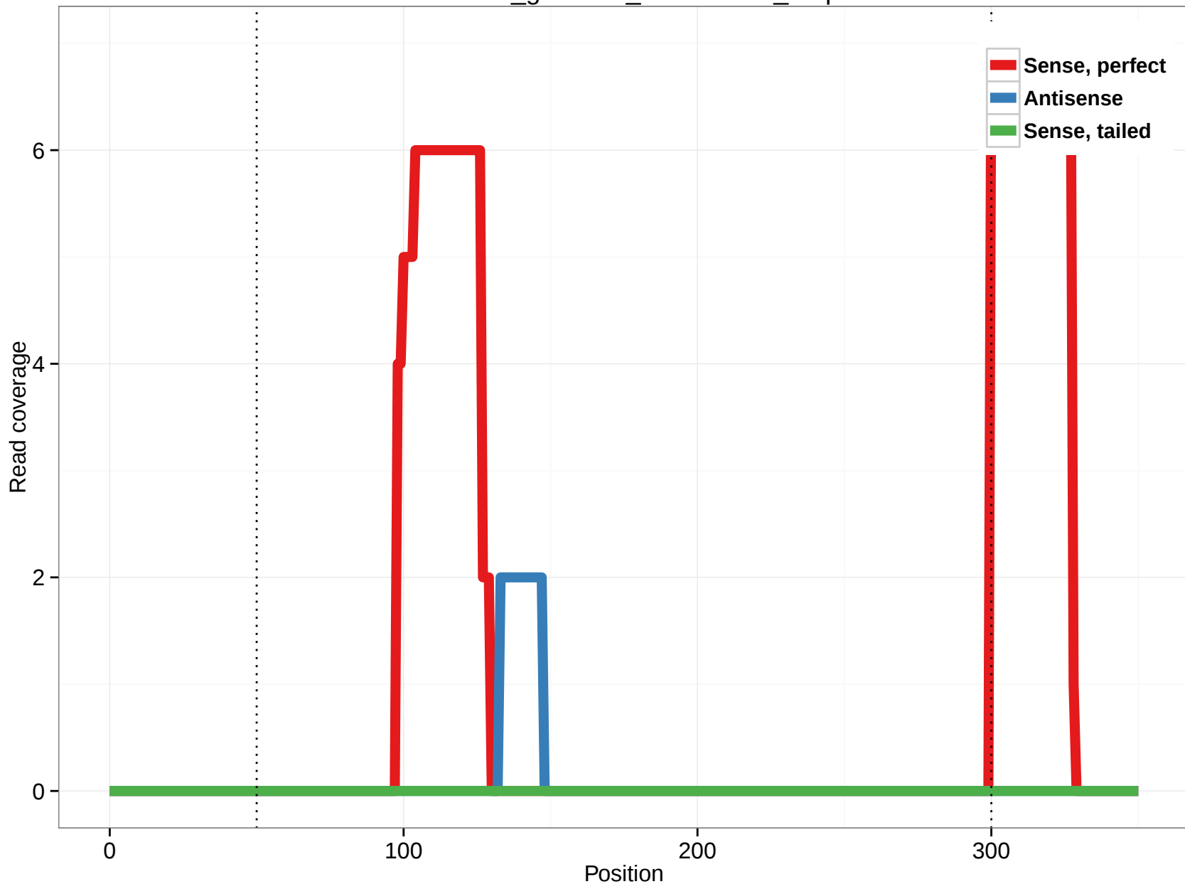
rheMac3_genscan_chr10.1562_3.5p
