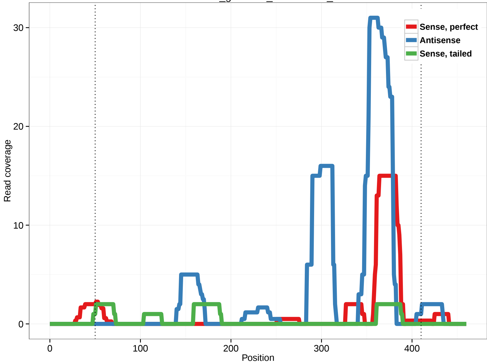
rheMac3_genscan_chr10.1553_1
