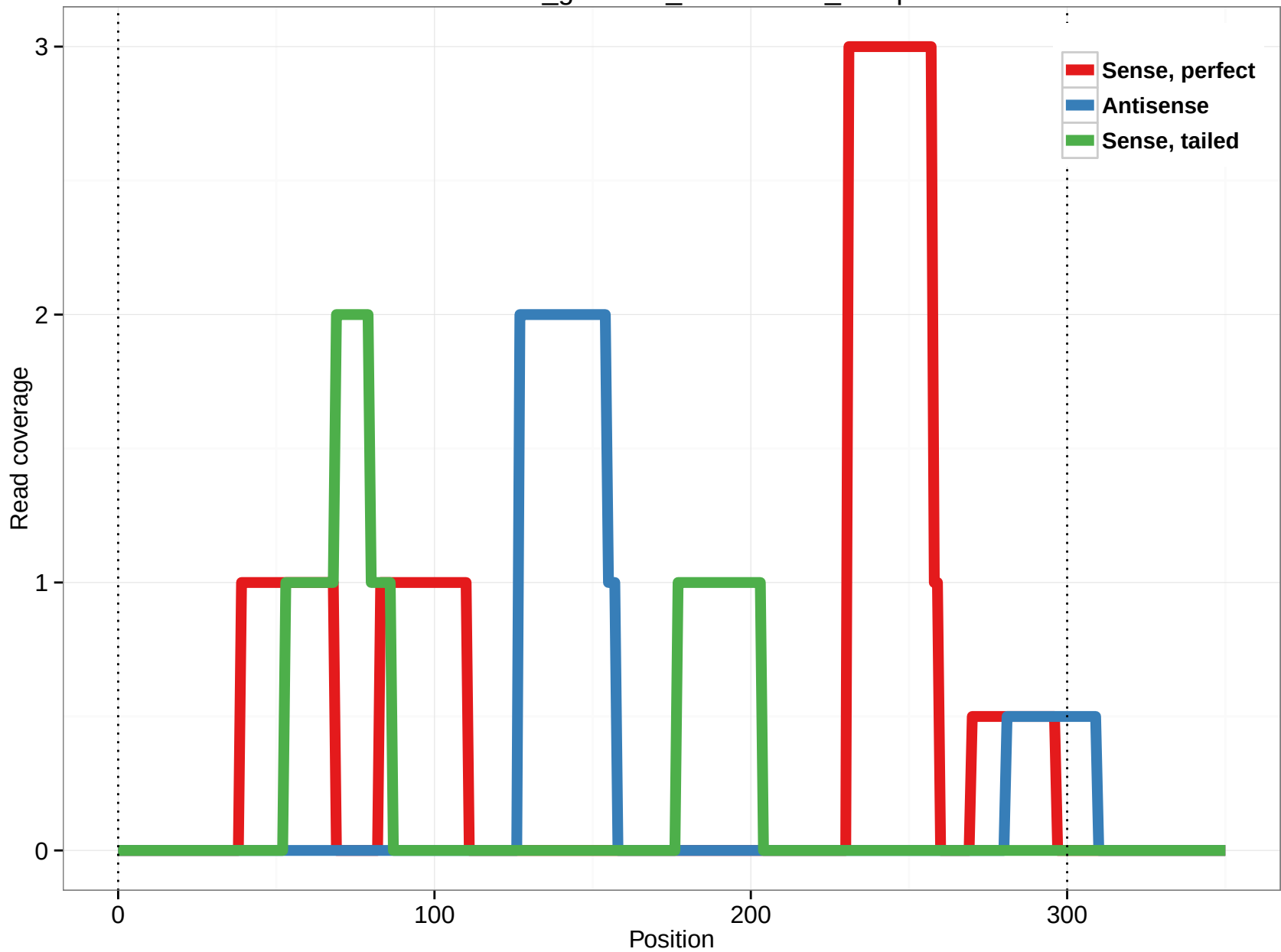
rheMac3_genscan_chr10.1552_26.3p
