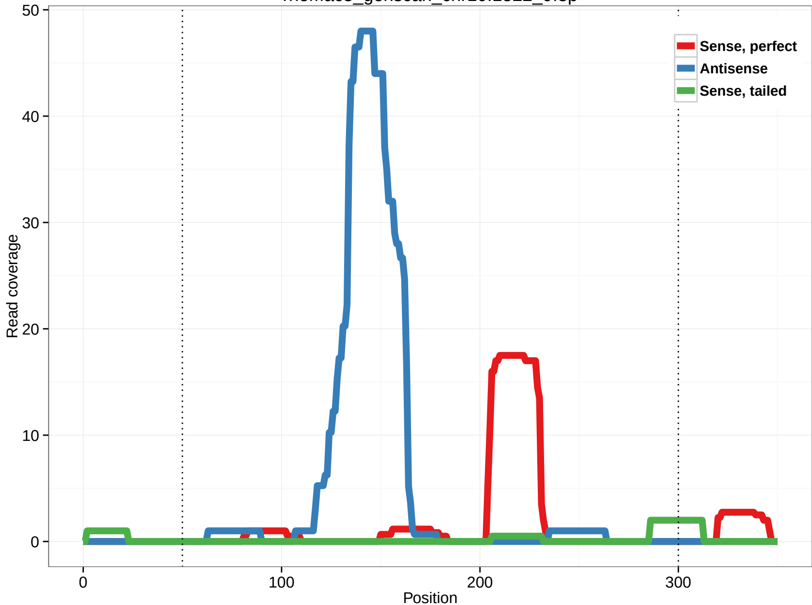
rheMac3_genscan_chr10.1522_9.3p
