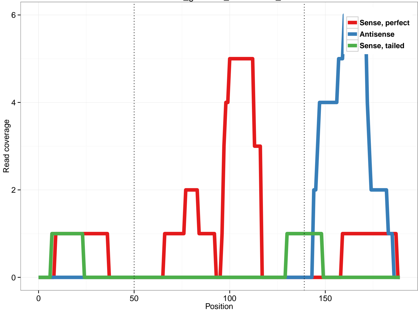
rheMac3_genscan_chr10.1509_23
