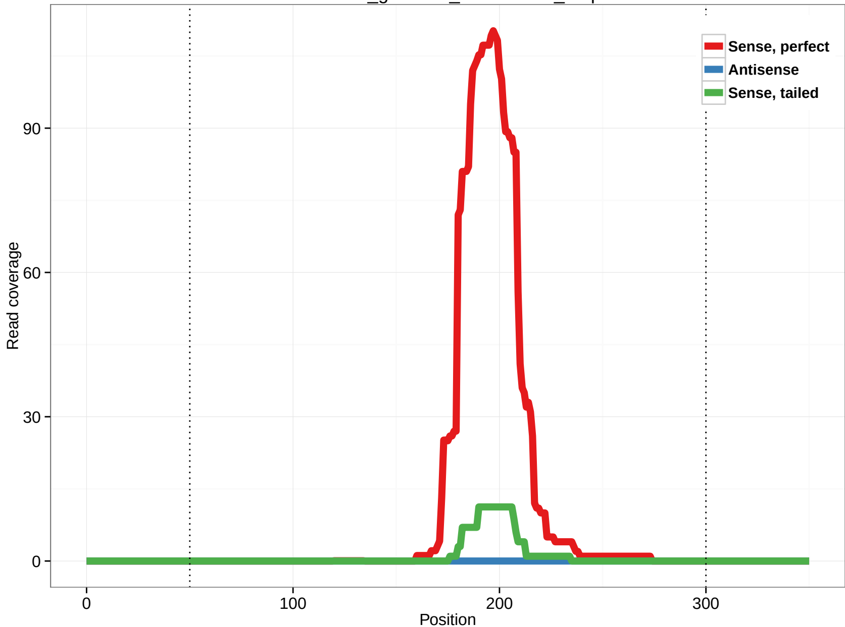
rheMac3_genscan_chr10.1497_2.3p
