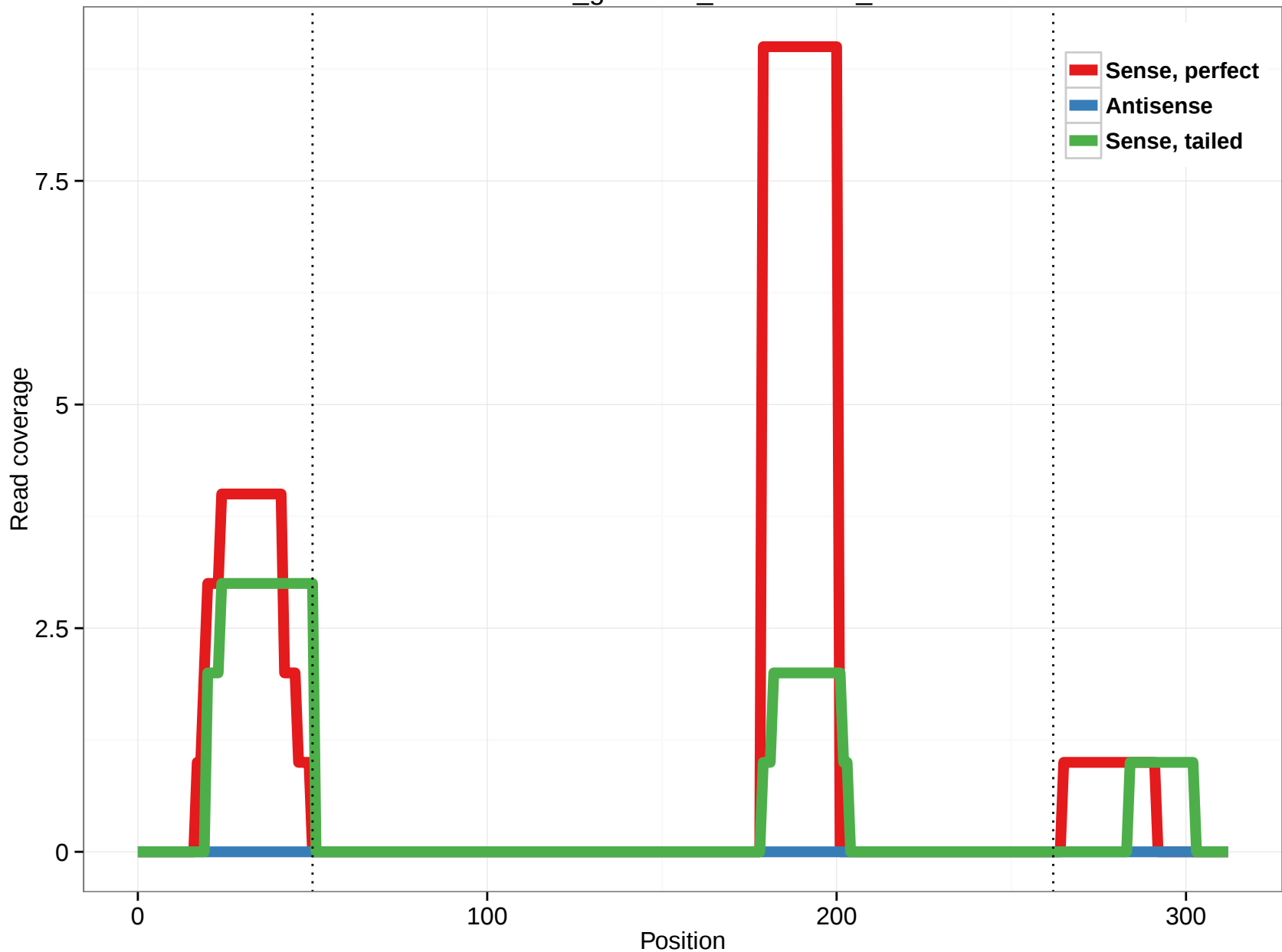
rheMac3_genscan_chr10.1496_11
