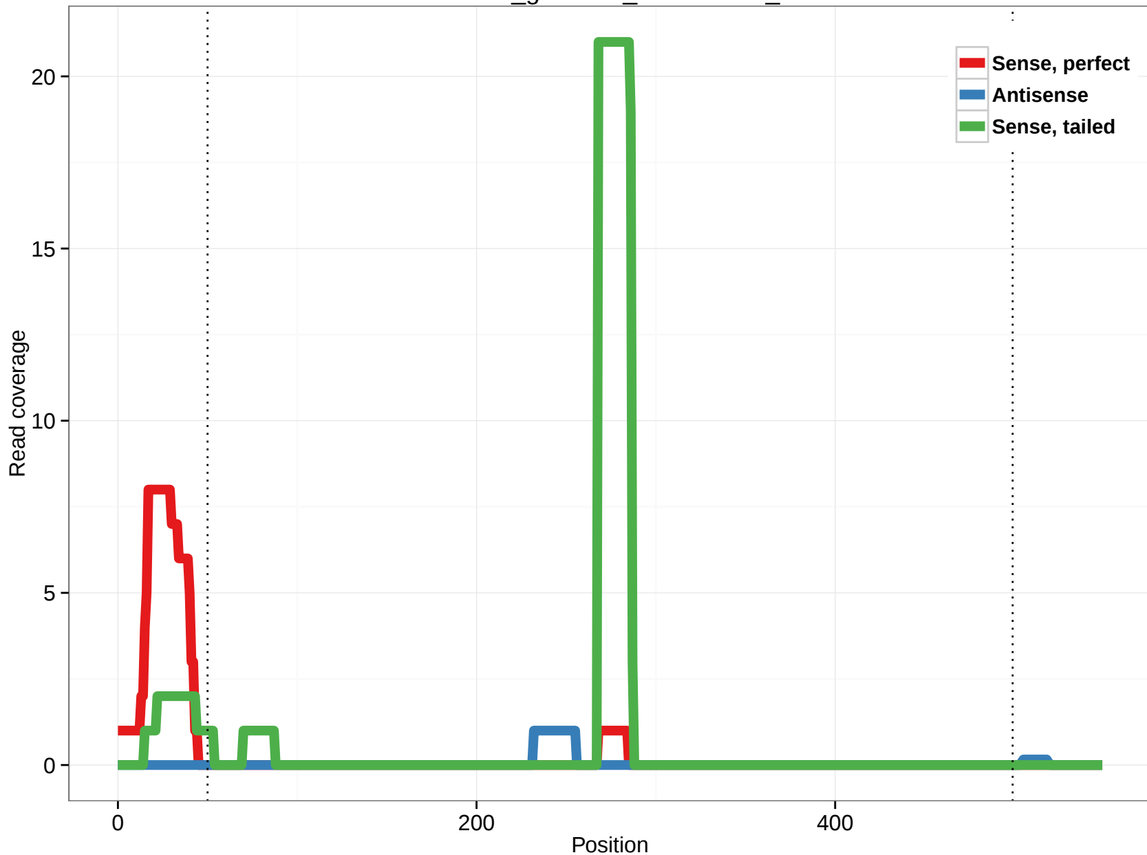
rheMac3_genscan_chr10.1496_10
