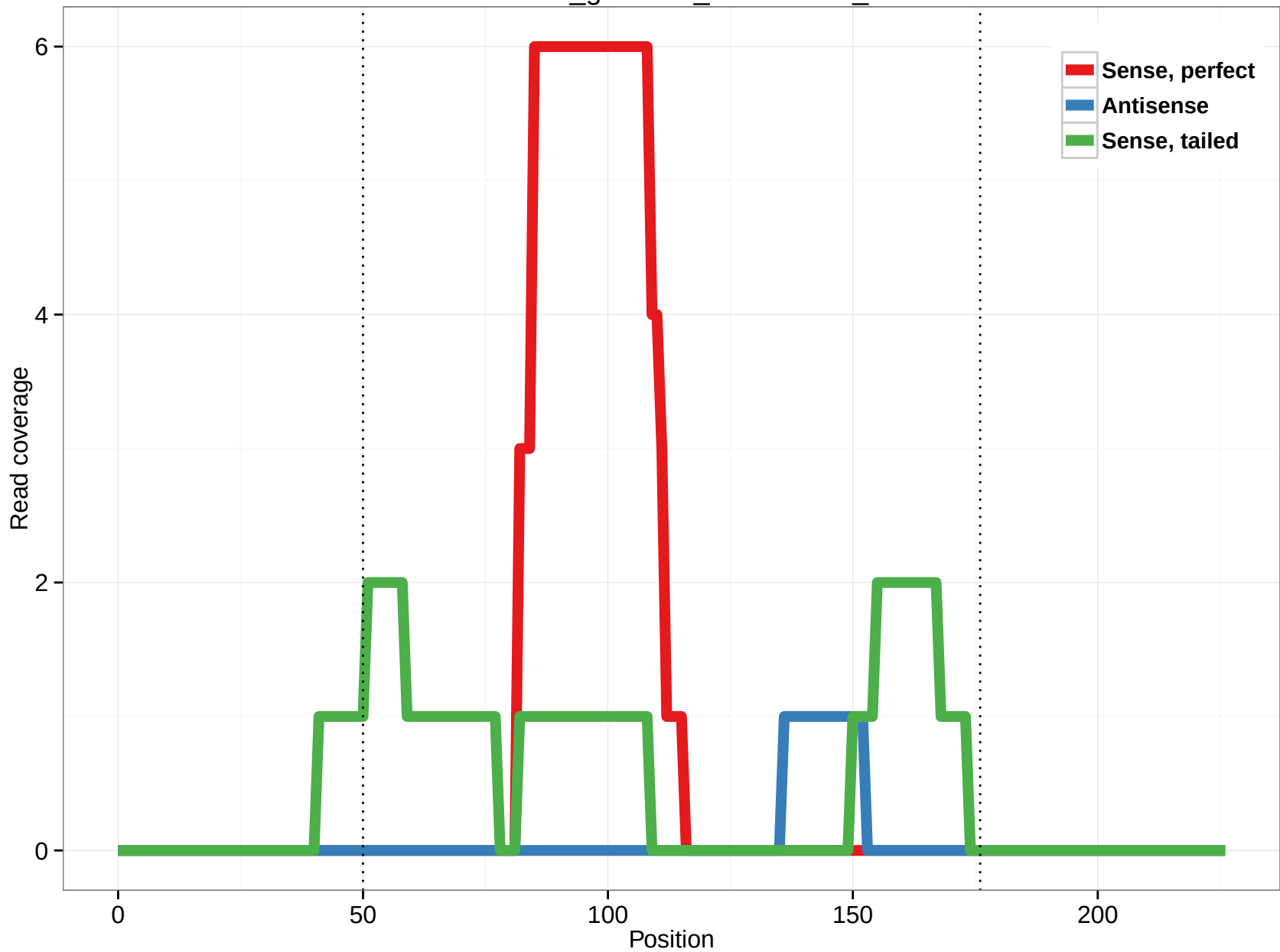
rheMac3_genscan_chr10.1456_3
