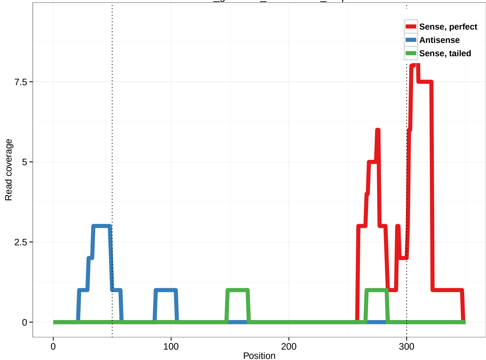
rheMac3_genscan_chr10.1455_0.5p
