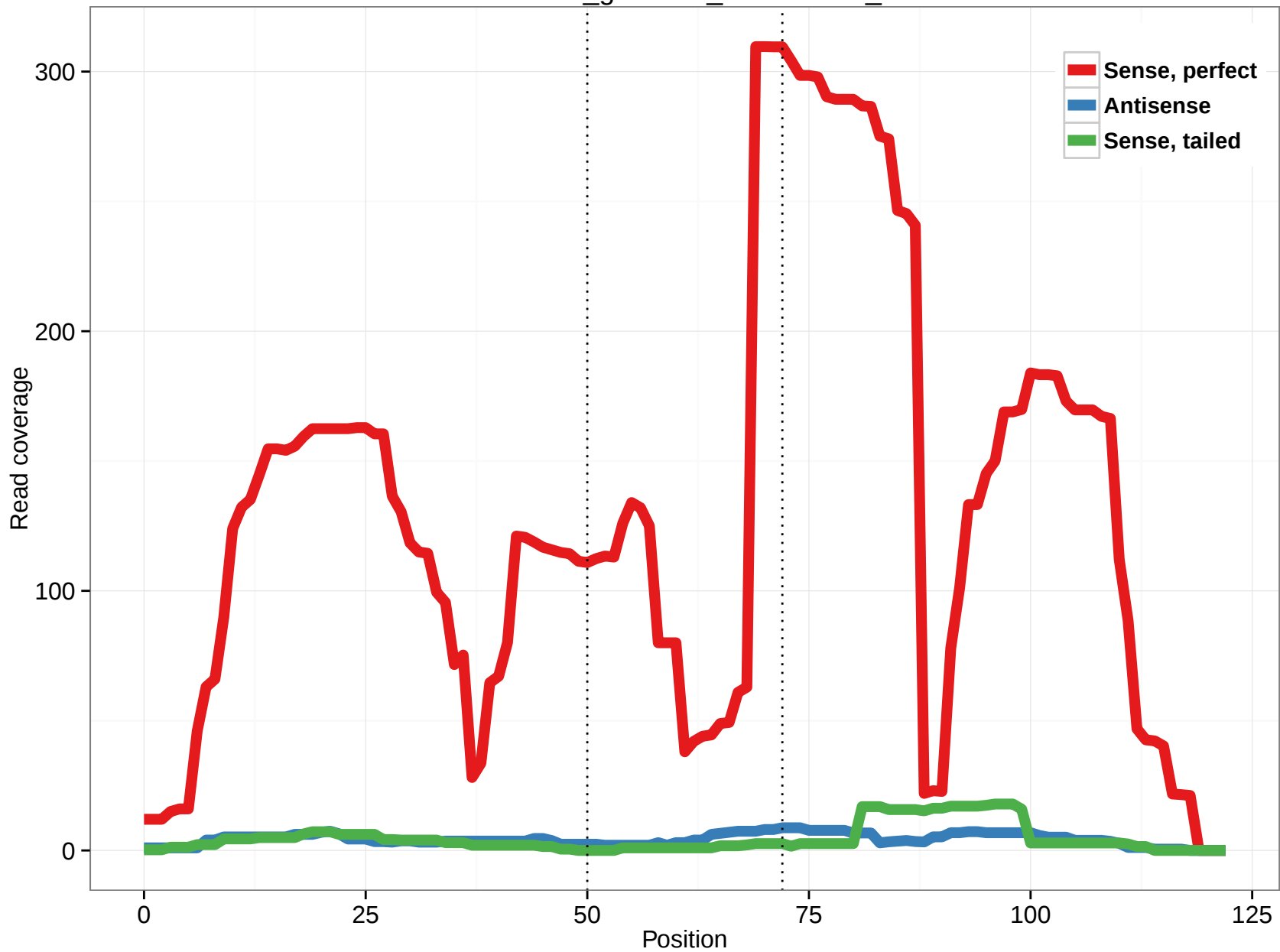
rheMac3_genscan_chr10.1453_1
