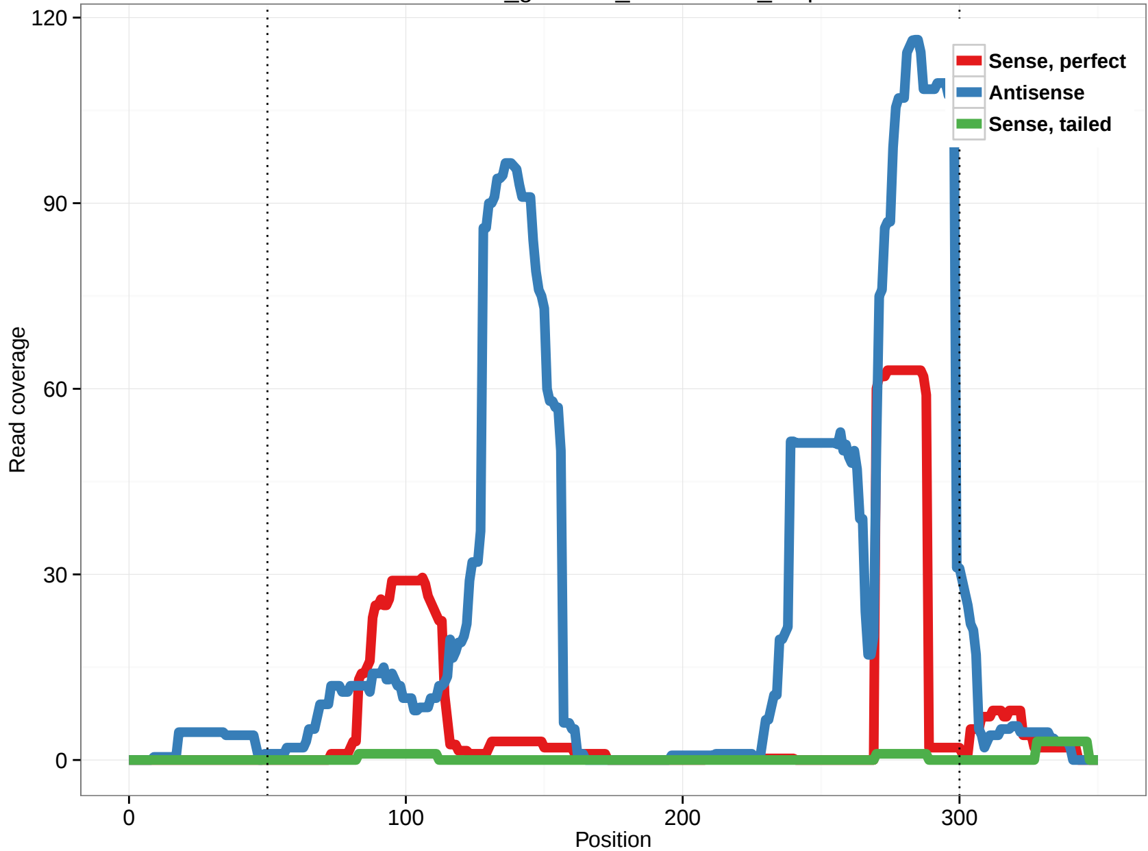
rheMac3_genscan_chr10.1453_0.3p
