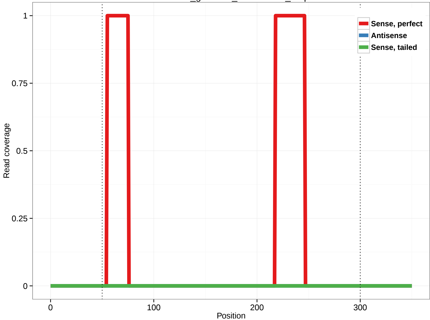
rheMac3_genscan_chr10.1441_0.3p
