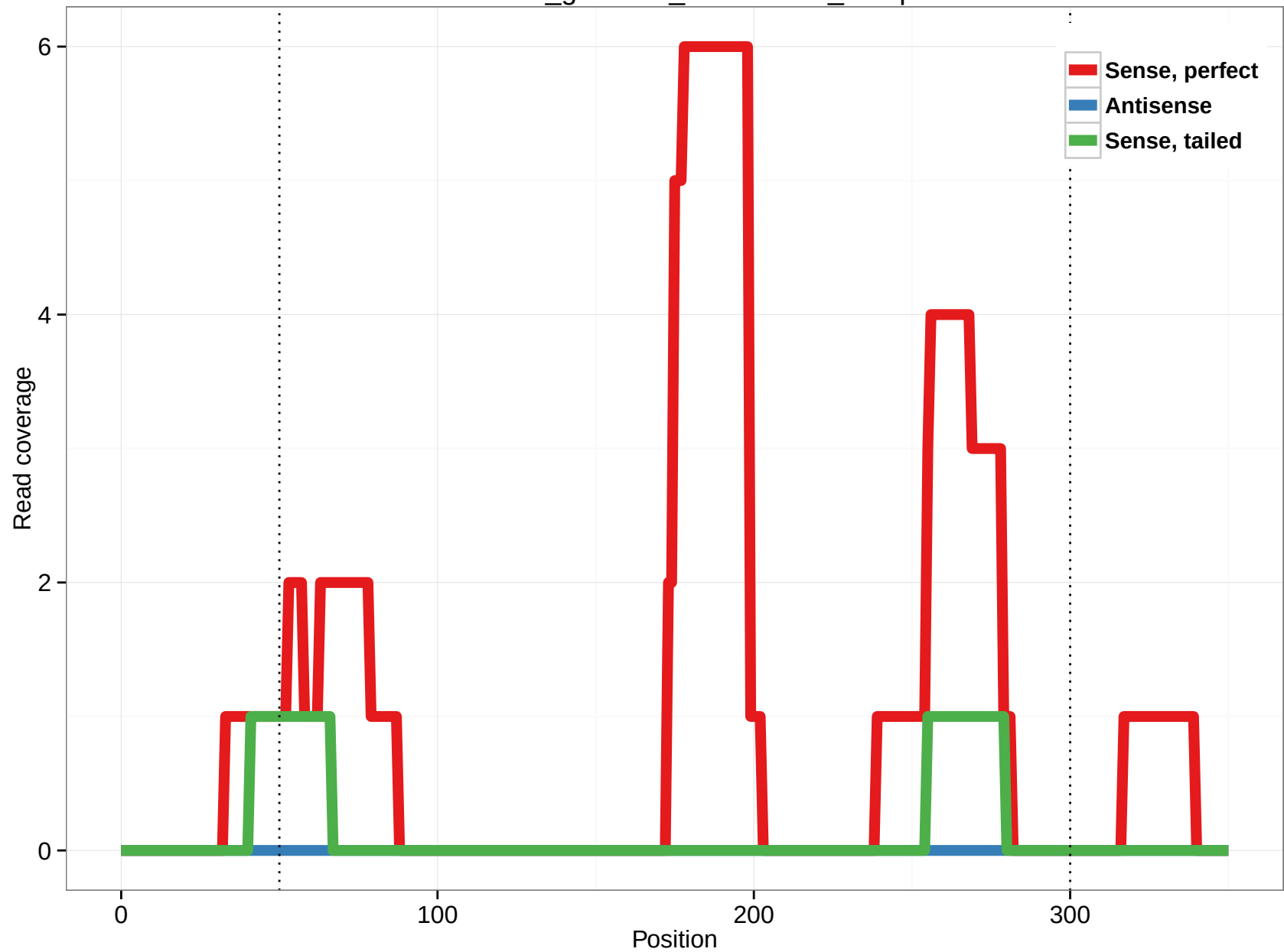
rheMac3_genscan_chr10.1386_48.5p
