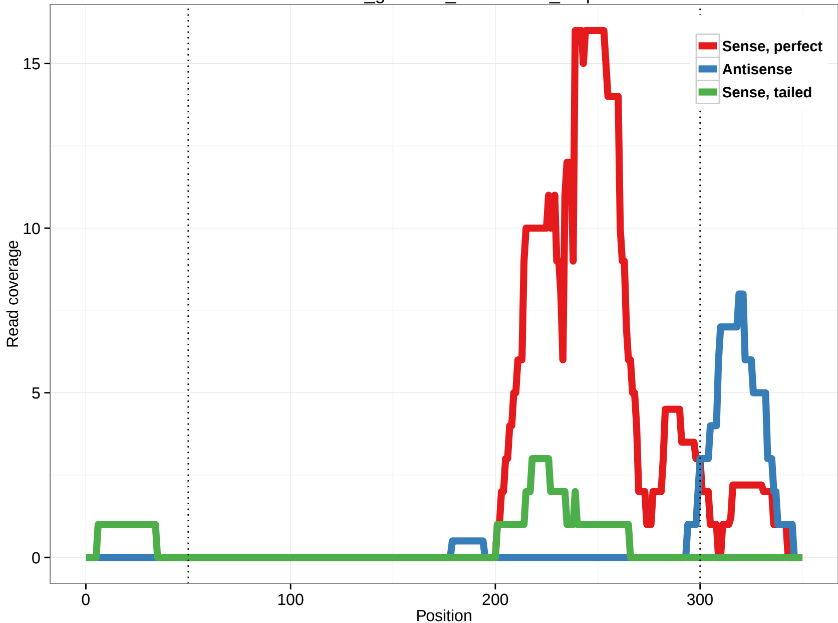
rheMac3_genscan_chr10.1385_4.3p
