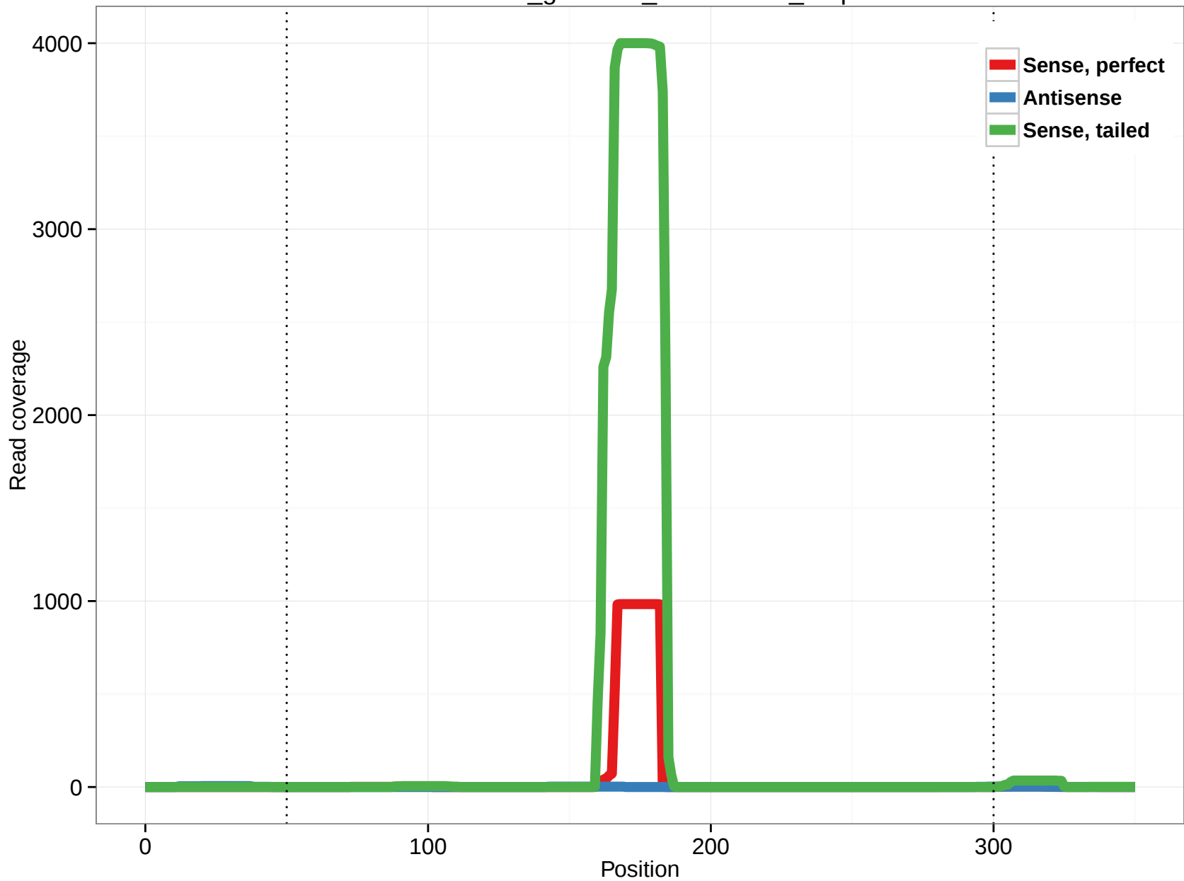
rheMac3_genscan_chr10.1358_2.3p
