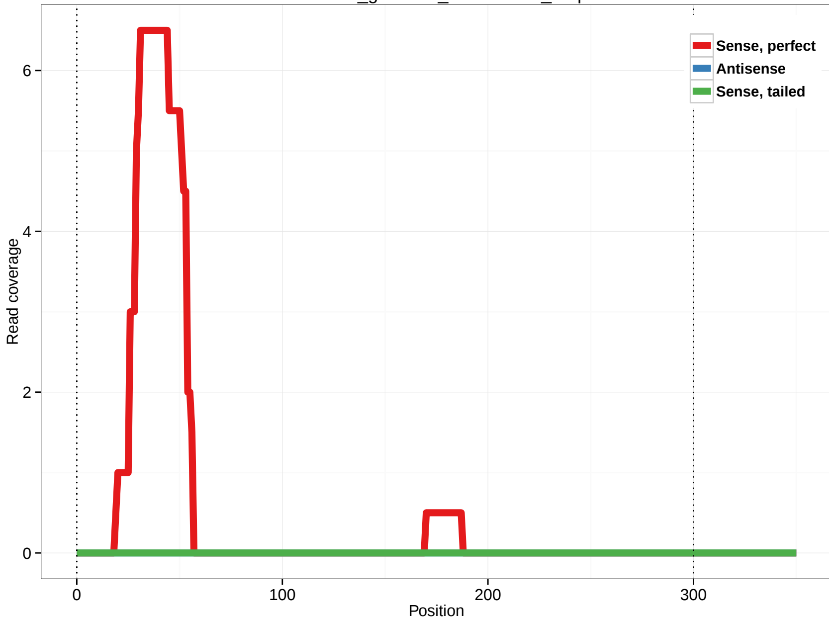
rheMac3_genscan_chr10.1357_5.3p
