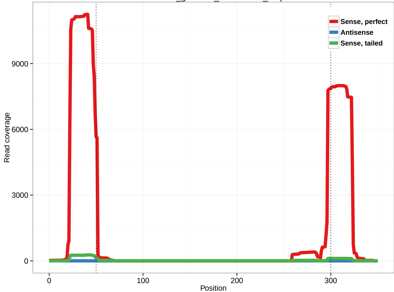
rheMac3_genscan_chr10.1357_4.3p
