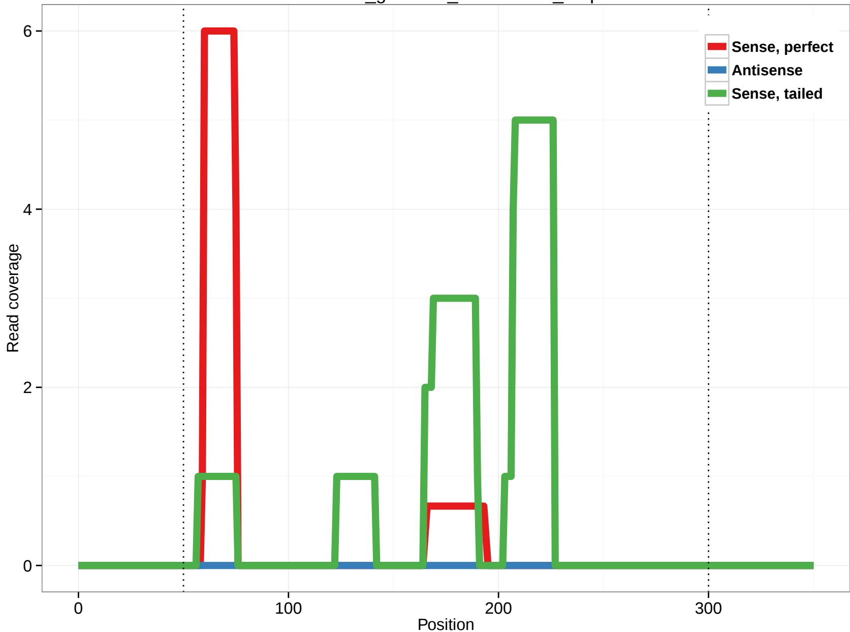
rheMac3_genscan_chr10.1345_3.3p
