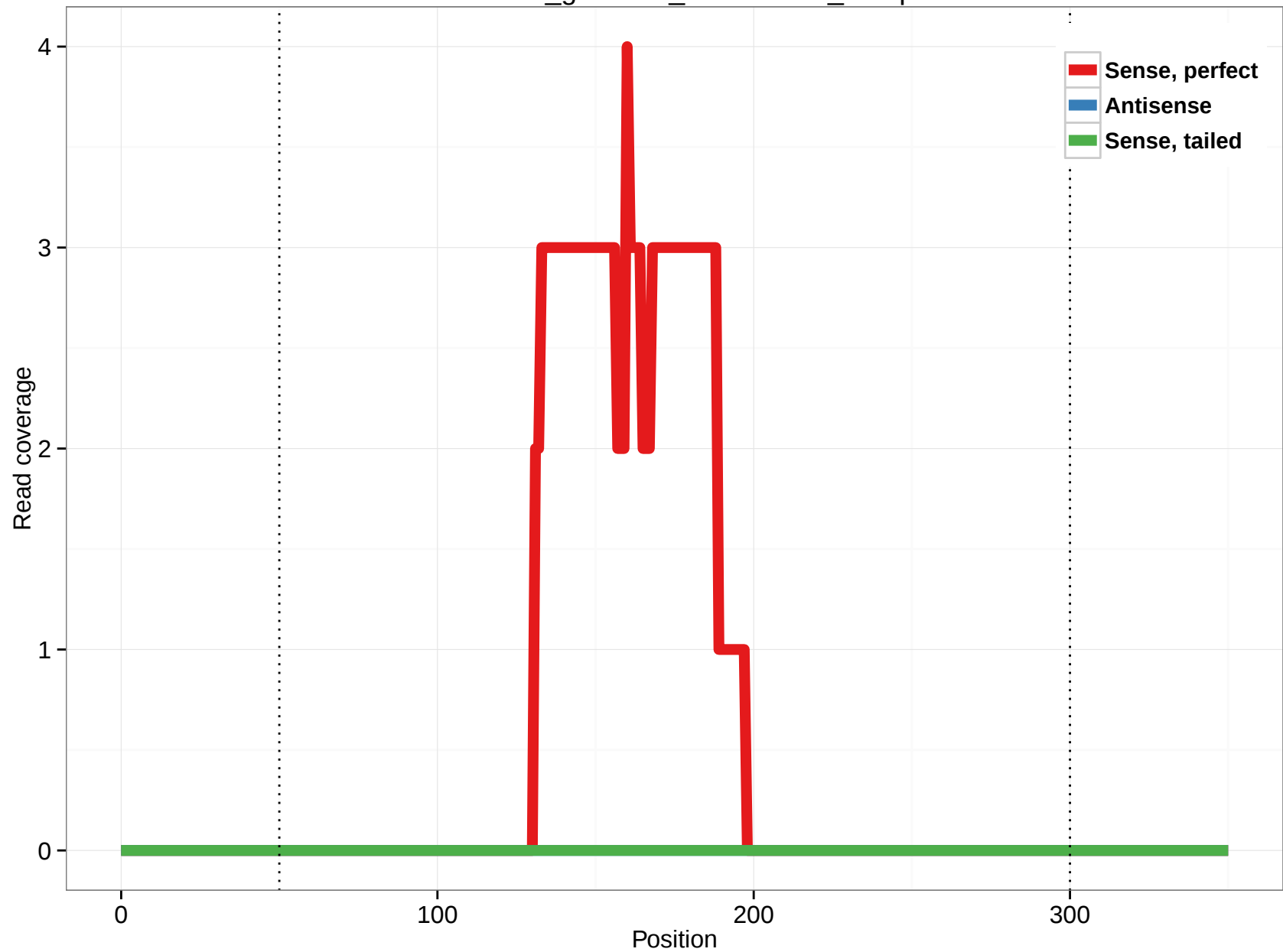
rheMac3_genscan_chr10.1343_26.5p
