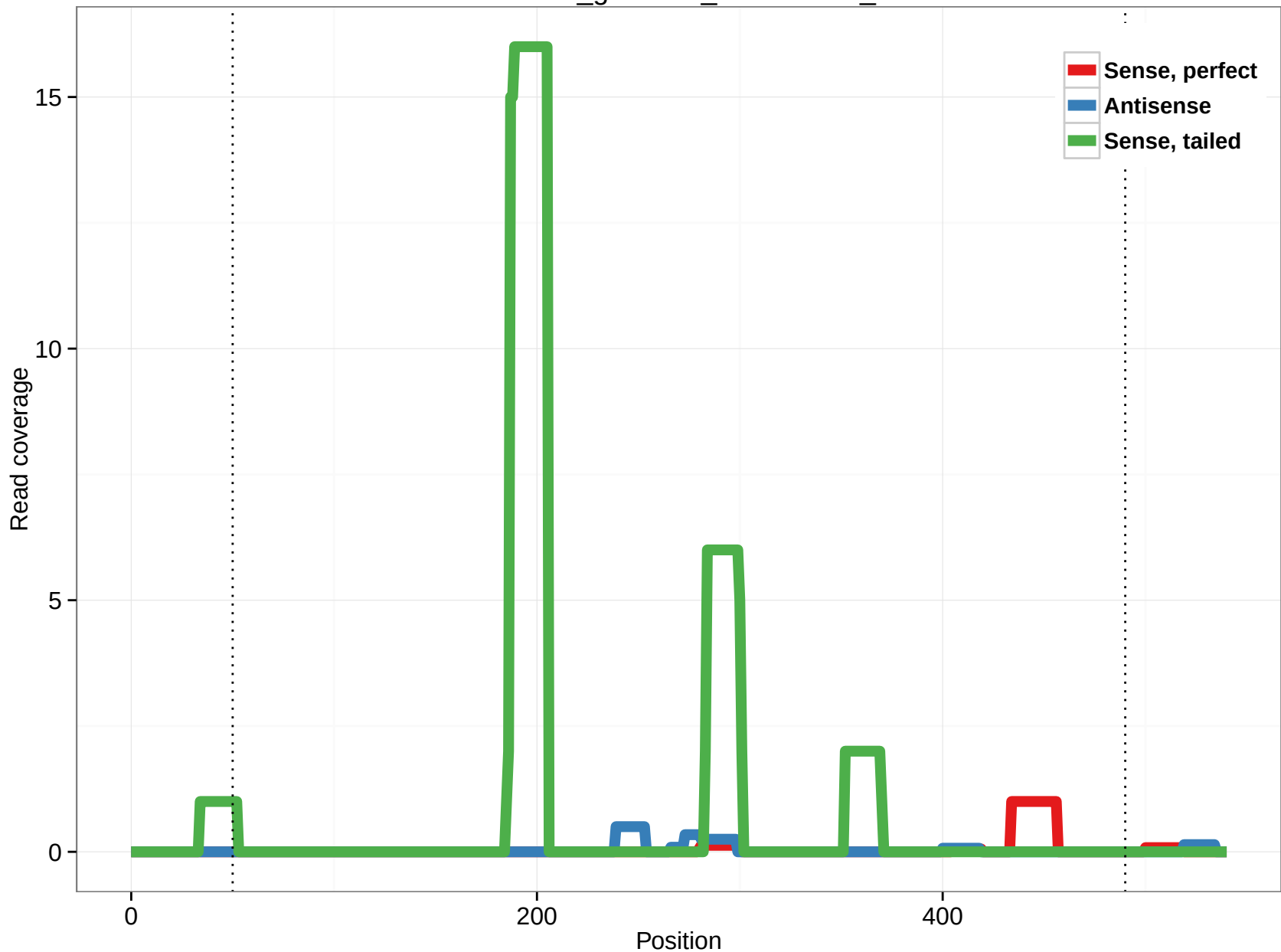
rheMac3_genscan_chr10.1288_1
