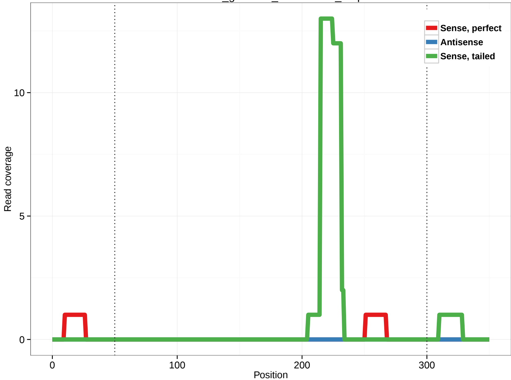
rheMac3_genscan_chr10.1177_7.5p
