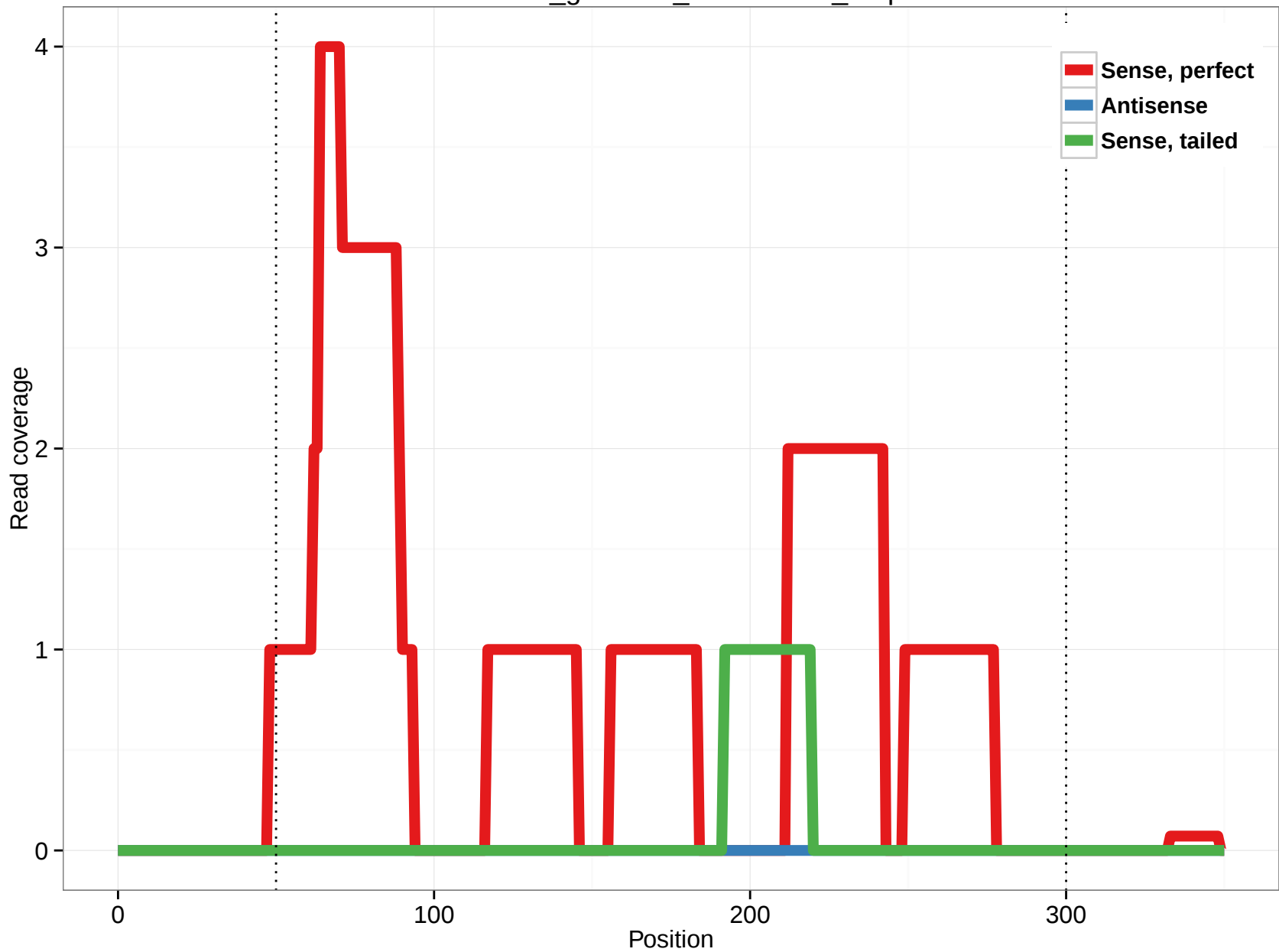
rheMac3_genscan_chr10.1166_7.5p
