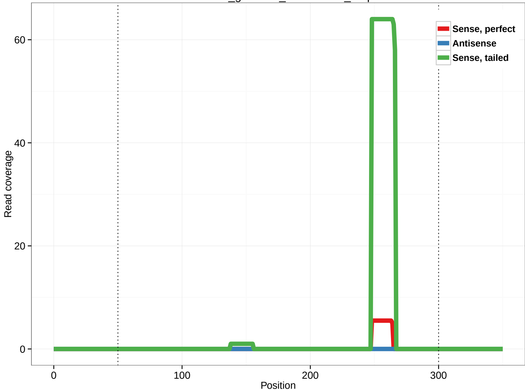
rheMac3_genscan_chr10.1142_3.3p
