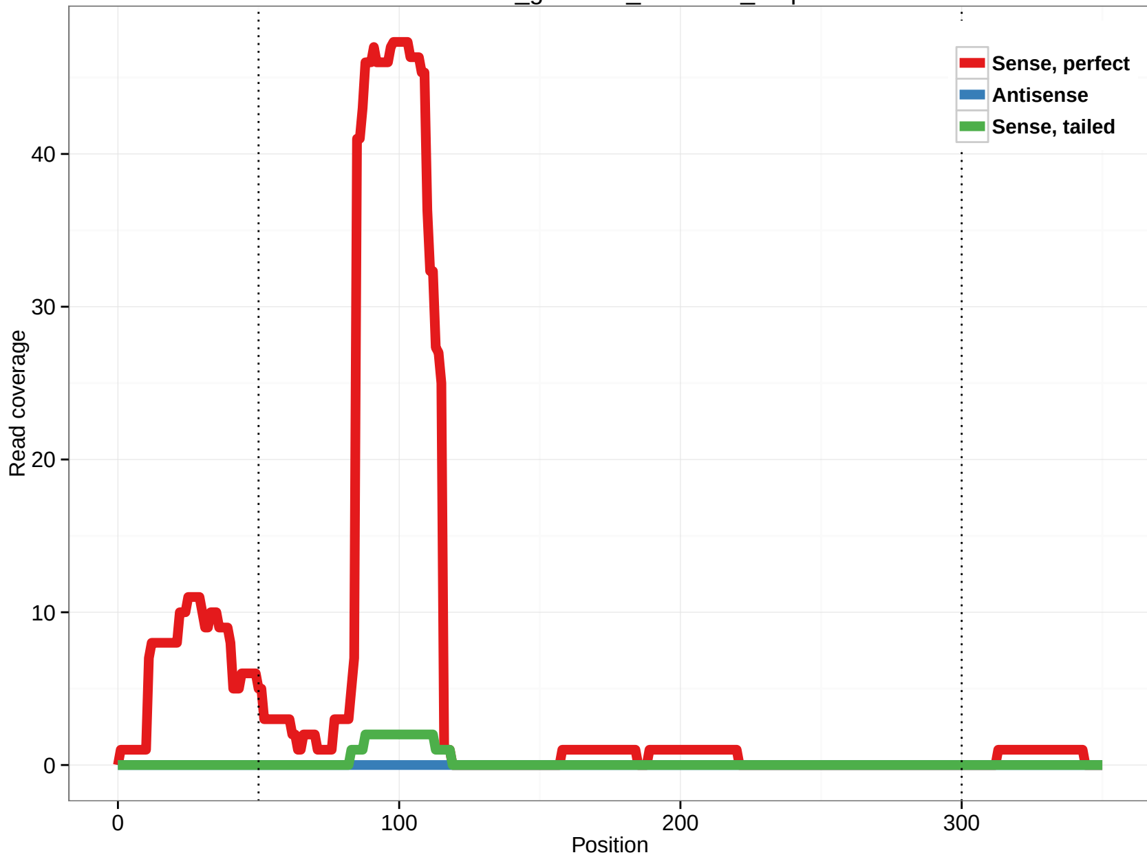
rheMac3_genscan_chr1.979_2.5p
