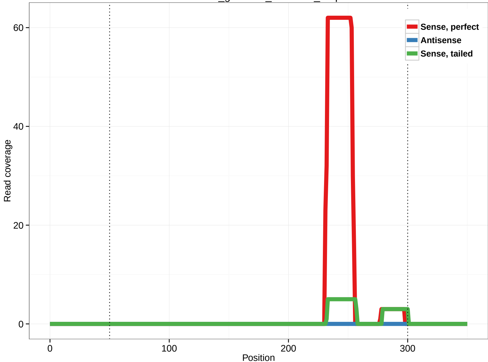
rheMac3_genscan_chr1.950_8.3p
