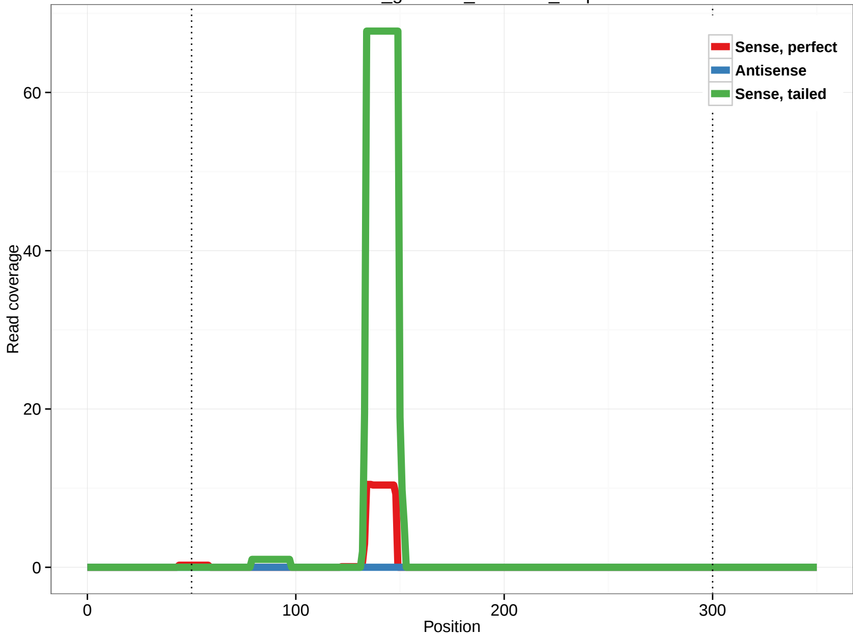
rheMac3_genscan_chr1.946_3.3p
