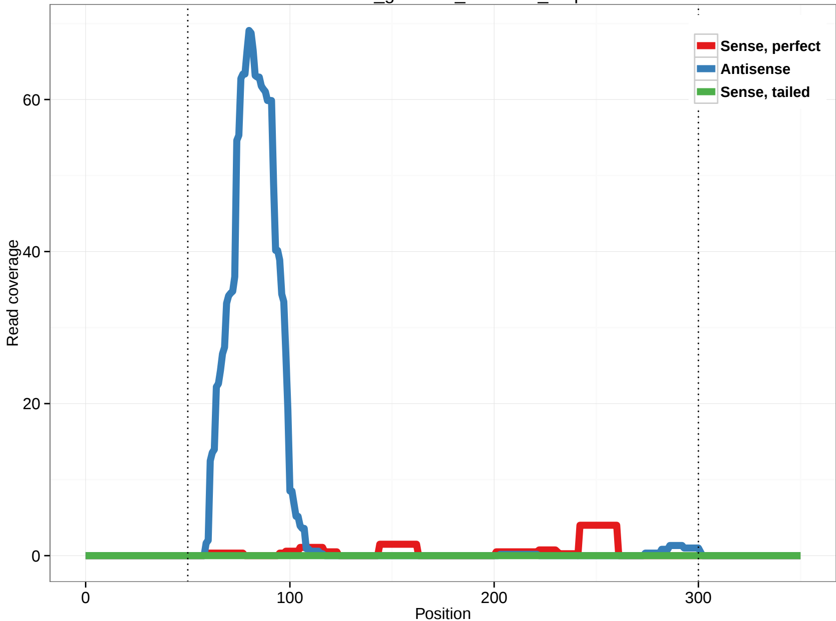
rheMac3_genscan_chr1.915_5.5p
