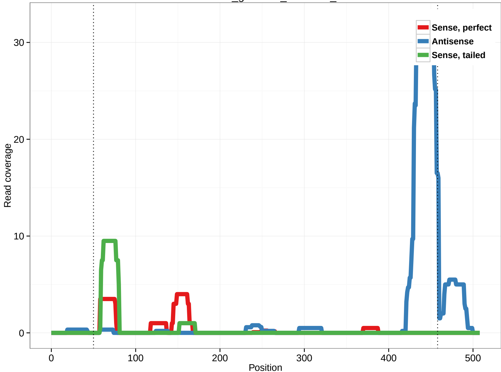
rheMac3_genscan_chr1.915_3
