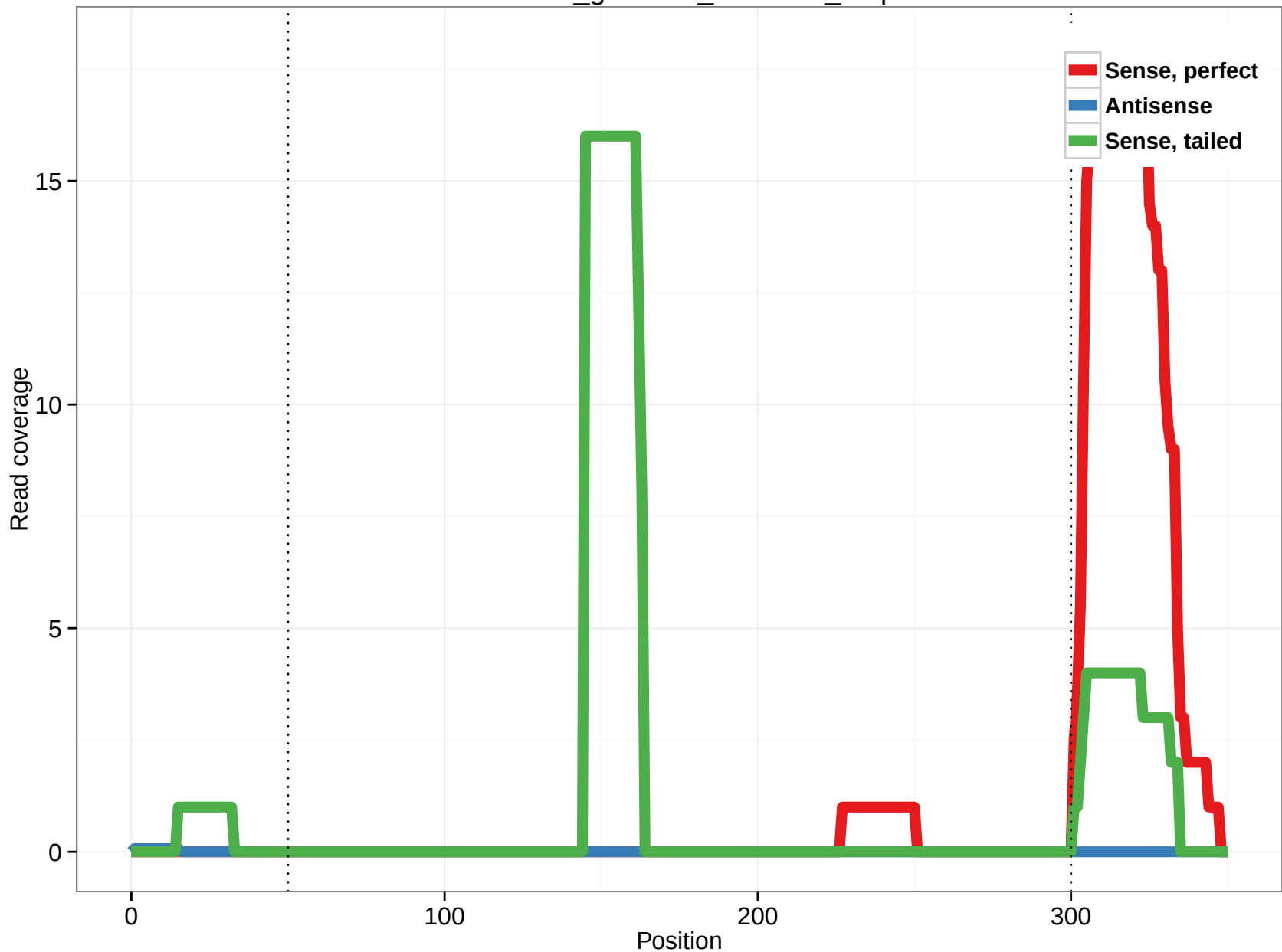
rheMac3_genscan_chr1.906_0.3p
