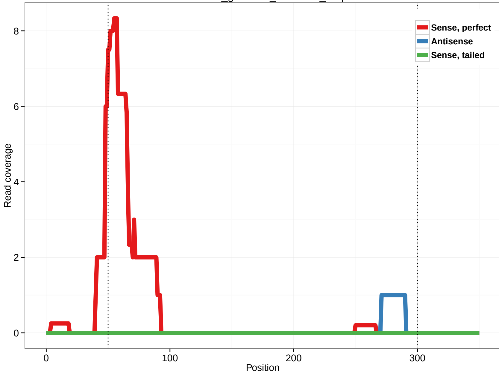
rheMac3_genscan_chr1.845_1.5p
