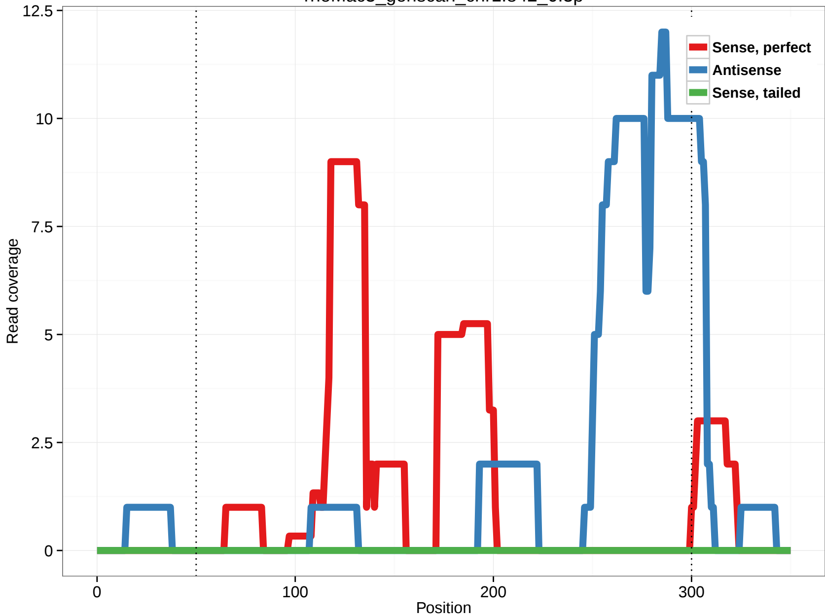
rheMac3_genscan_chr1.842_0.3p
