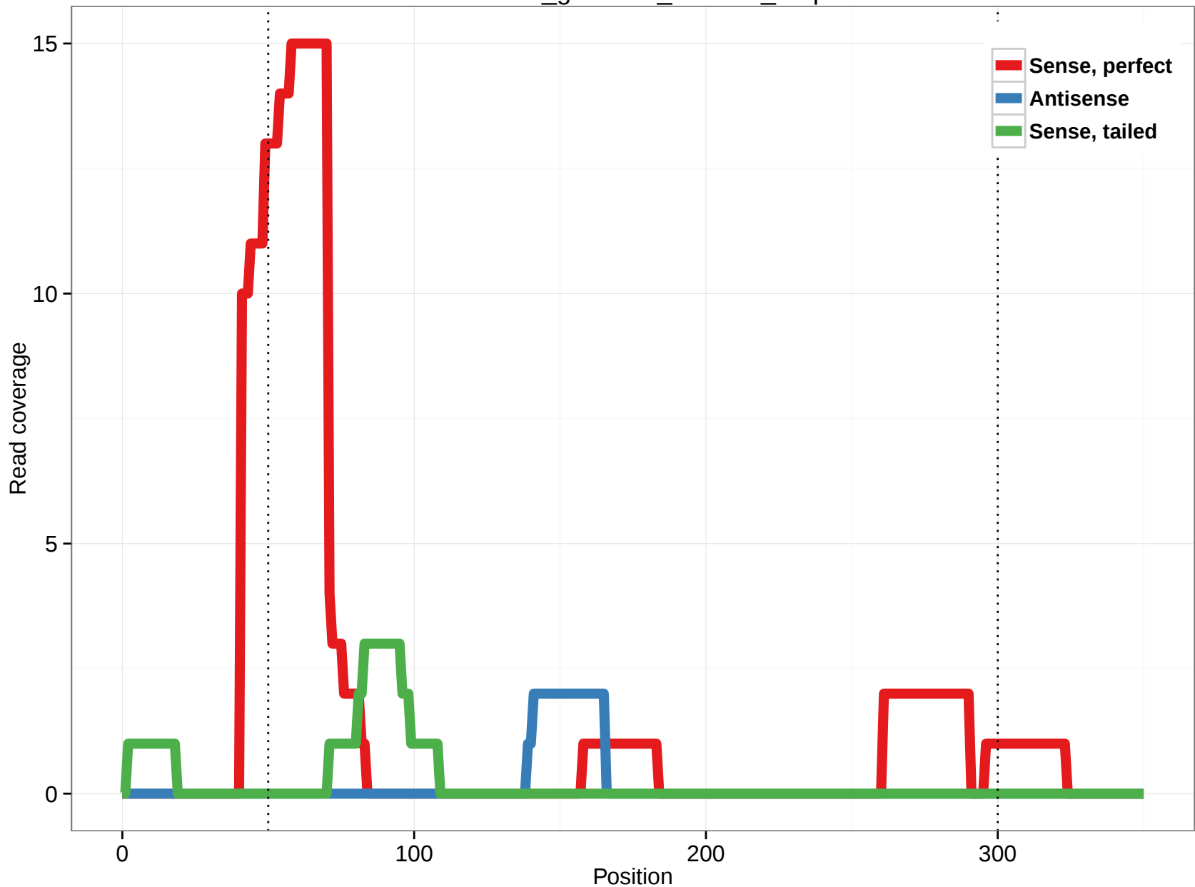
rheMac3_genscan_chr1.83_6.3p
