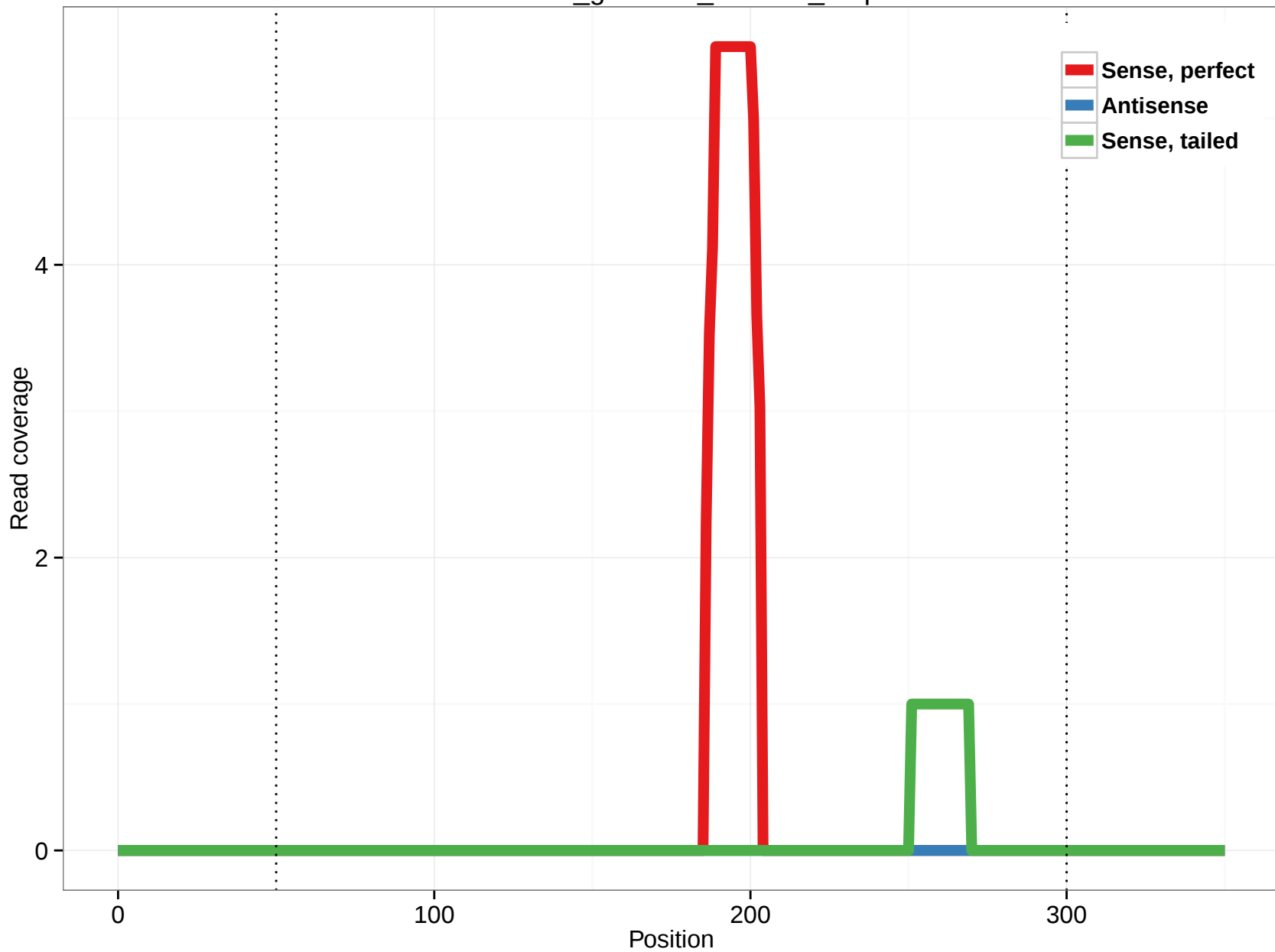
rheMac3_genscan_chr1.79_0.5p
