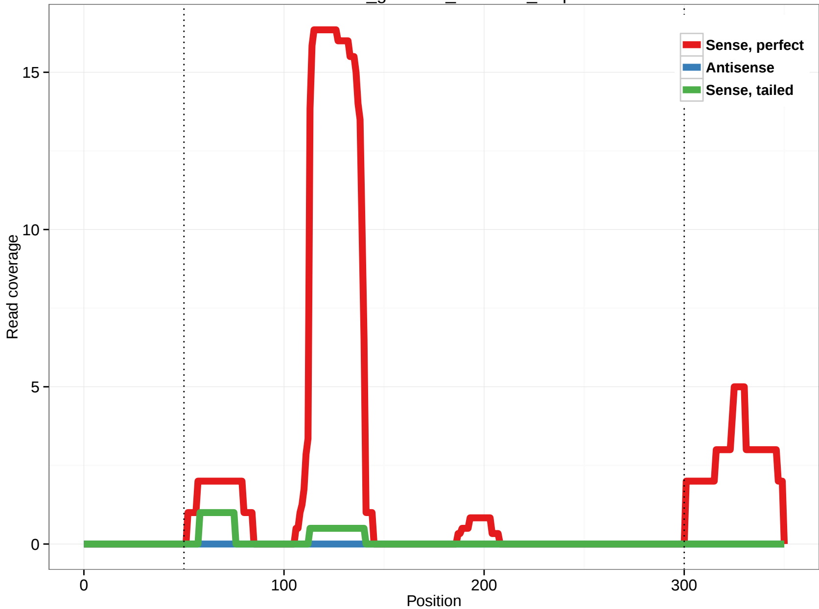
rheMac3_genscan_chr1.799_3.3p
