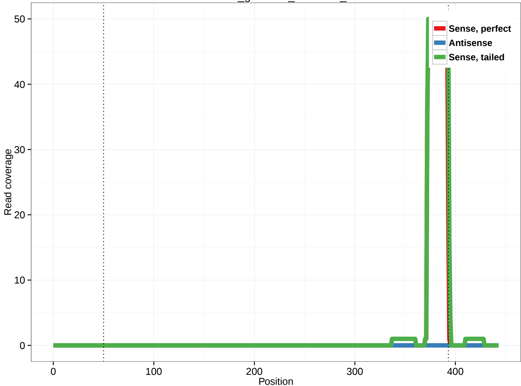
rheMac3_genscan_chr1.793_10
