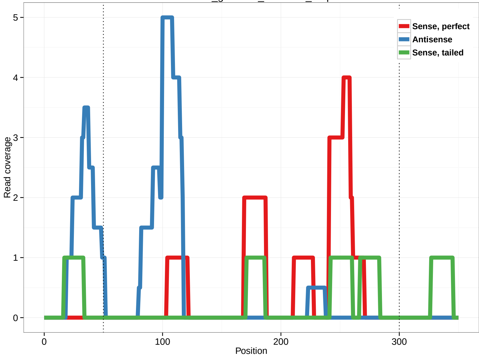
rheMac3_genscan_chr1.765_0.5p
