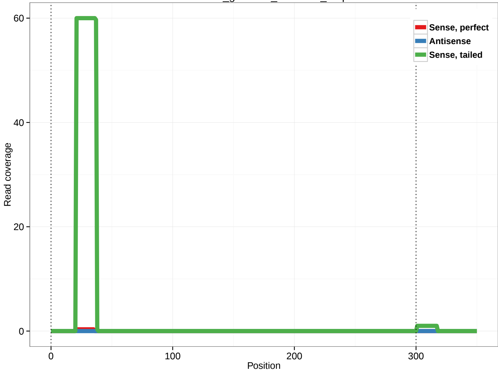
rheMac3_genscan_chr1.757_2.3p
